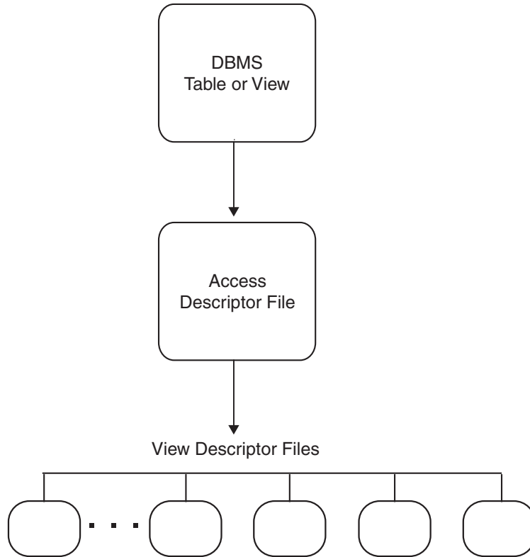
Figure 14.1 Creating an Access Descriptor and View Descriptors for a DBMS Table
